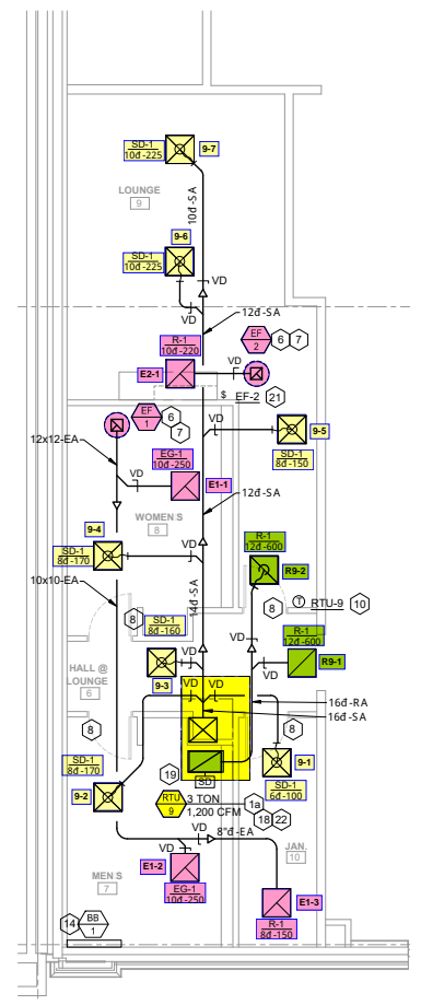
04 ENLARGED MECHANICAL PLAN-LOUNGE AREA
